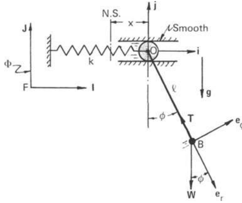
Figure 6.19. Motion of a pendulum having a moving support.
