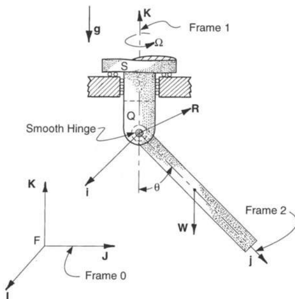
Figure 10.11. Spatial motion of a rigid rod hinged to a rotating shaft.
