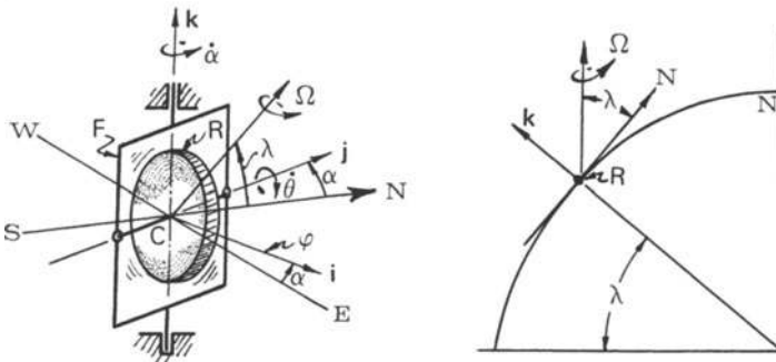
Figure 10.12. Schematic model of a gyrocompass.
