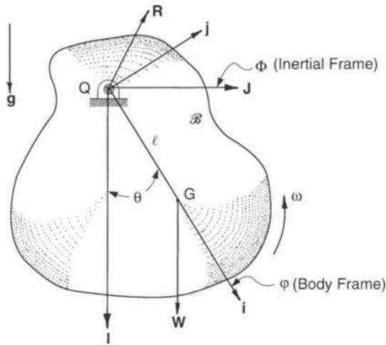
Figure 10.15. Oscillation of a physical pendulum.
