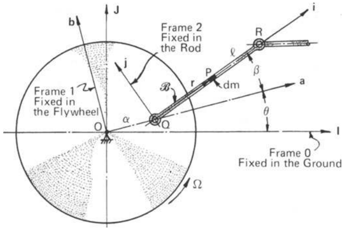
Figure 10.6. Moment of momentum about a moving point Q in a simple machine.
