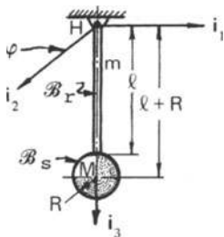
Figure 9.9. Application of the parallel axis theorem to a composite pendulum.
