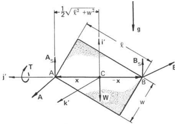
Figure 10.10. Free body diagram of the rotating plate.
