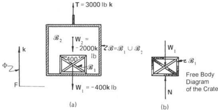
Figure 10.3. Forces on a rigid crate in a moving elevator.
