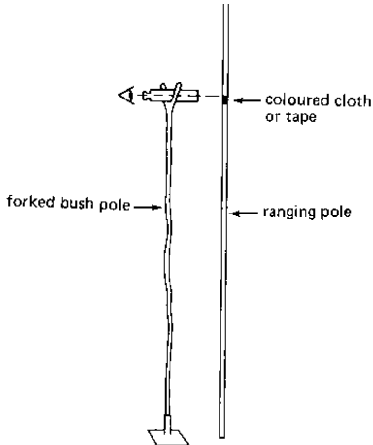
Fig. 49b Setting out a contour line, Step 2
