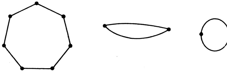
Fig. 2-9 Three different circuits.
