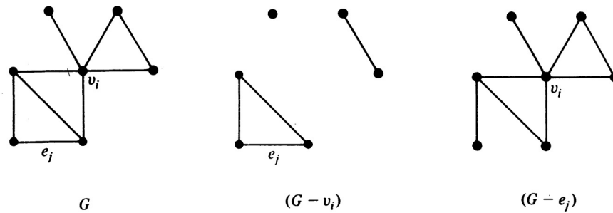
Fig. 2-15 Vertex deletion and edge deletion.
