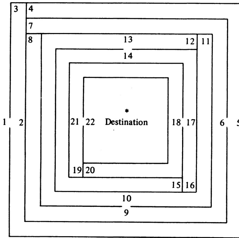
Fig. 1-13 A maze.
