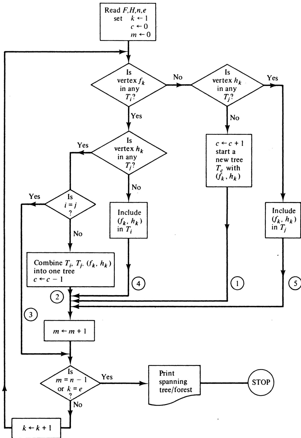
Fig. 11-3 Algorithm 2: Spanning tree/forest.
