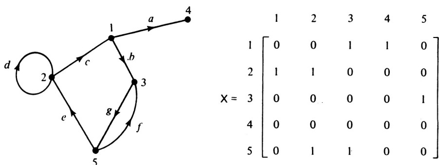
Fig. 9-19 Digraph and its adjacency matrix.
