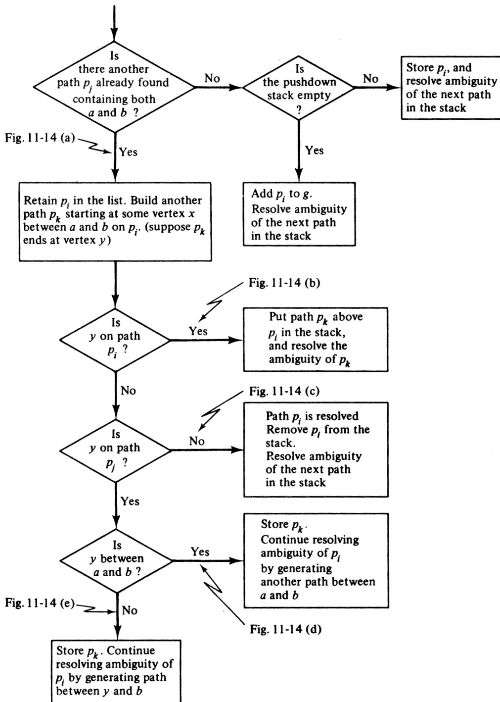
Fig. 11-14 Resolution of ambiguity of path p_i .
