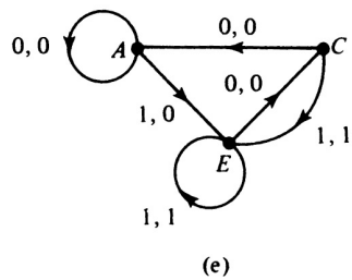
Fig. 12-8 Reduction of a state graph.
