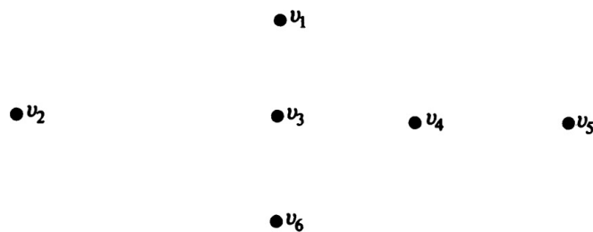
Fig. 1-12 Null graph of six vertices.
