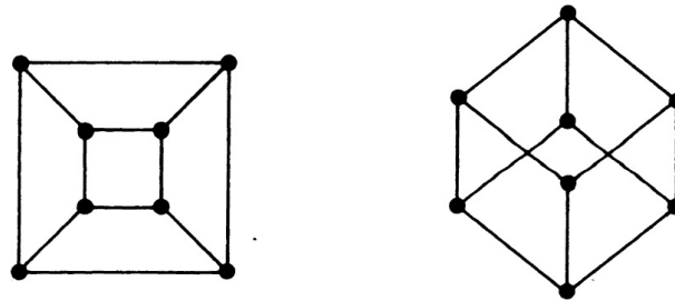
Fig. 2-2 Isomorphic graphs.
