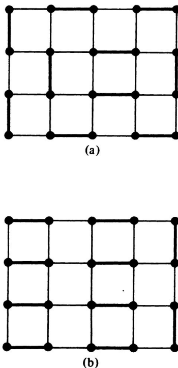
Fig. 8-13 Two dimer coverings of a graph.
