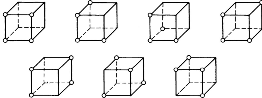
Fig. 10-9 Attaching four balls to corners of a cube.
